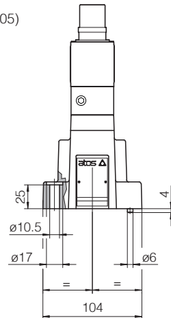
AGRCZO-AEB-NP-20 AGRCZO-AEB-IL-20 standard and /R
