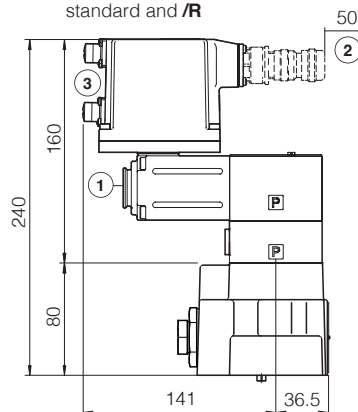
AGRCZO-AES-BC-10 AGRCZO-AES-BP-10 standard and /R
