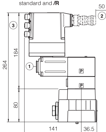
AGRCZO-AES-EH-10 standard and /R
