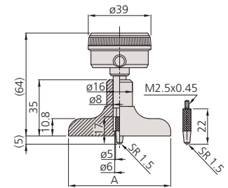
7237, 7231 A=63.5mm 7238 A=101.6mm
