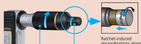
Ratchet on thimble Ratchet on speeder
