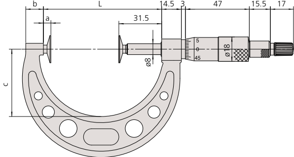
Analog model
